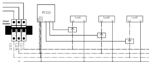
3-Phase Electricity Wiring Diagram
